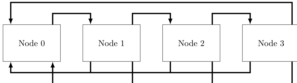
Figure 3.3: Decentralized Daisy-chain
